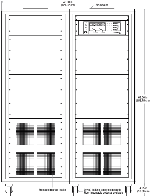
Front Side 150 kW Models
