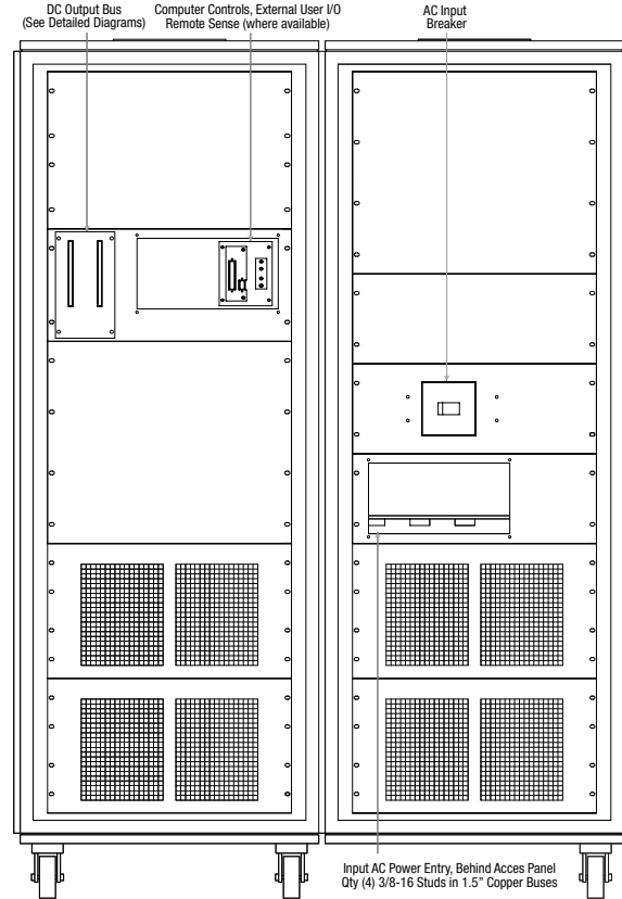
Rear Side 150 kW Models
